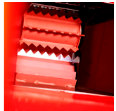
Dual Torque. Horizontal rollers with 8" roller opening (8.5 x 10.4")
